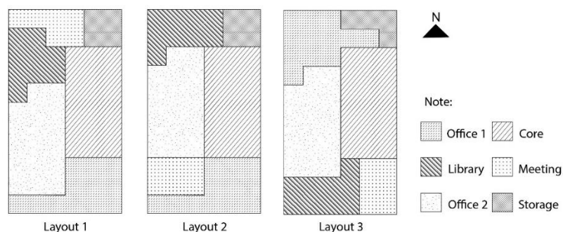
Figure 7. Three layouts with similar WWRs in [68]. The interior partitions divide the layout into different thermal zones.
