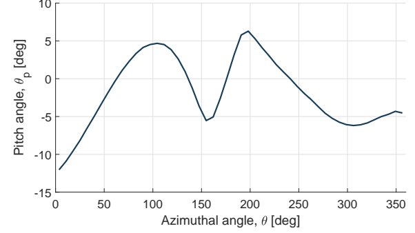
(f) Min C_x - Pitch schedule
