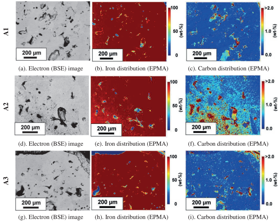
Fig. 6.4 EPMA (Electron Probe Micro-analyser) scan at location A1, A2 and A3 from Figure 6.3.
