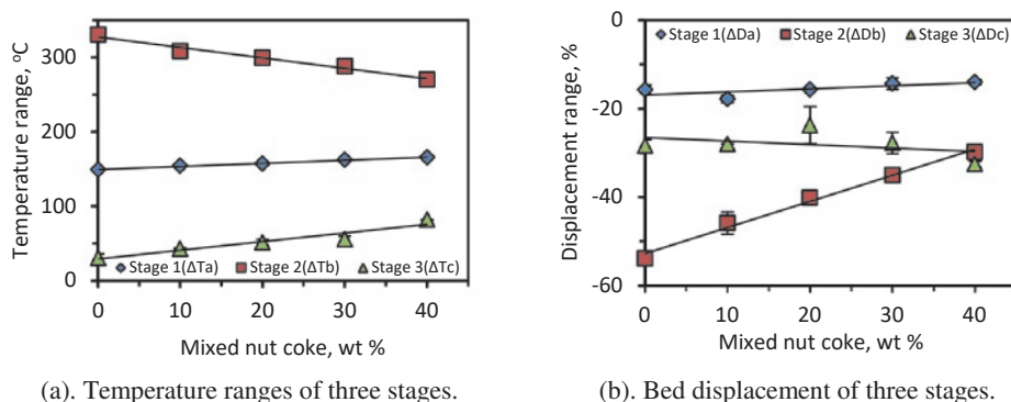
Fig. 5.7 Effect of nut coke on bed displacement and temperature ranges of different stages.
