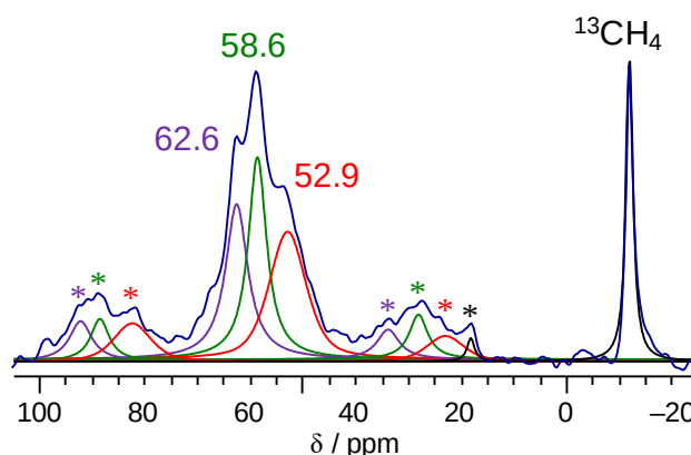
Figure 1. ^{13}\text{C} CP/MAS NMR spectrum of surface intermediates formed from methane- ^{13}\text{C} adsorbed on a Cu-ZSM-5 zeolite. The sample was spun at 3.0 kHz. Asterisks (*) indicate spinning side bands.
