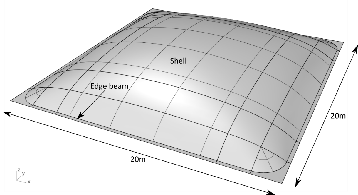
Figure 6 Surface model after reverse engineering of the point cloud
