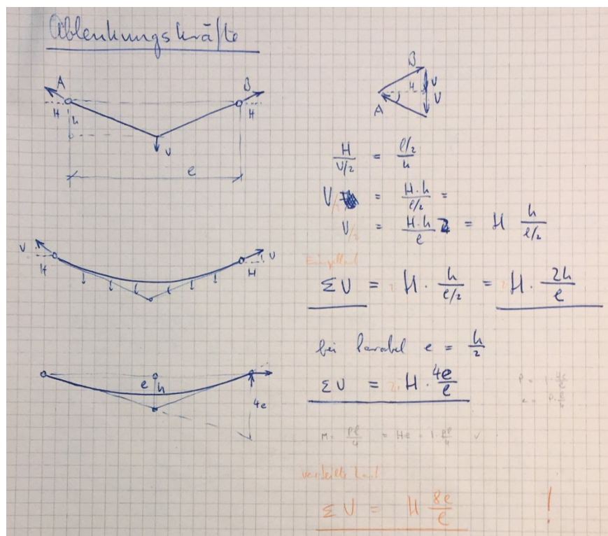
Figure 10 Derivation of forces in a pre-tensioned cable by H. Isler (Photo: Eigenraum taken from © gta Archives / ETH Zurich, Heinz Isler Archive - 217)
