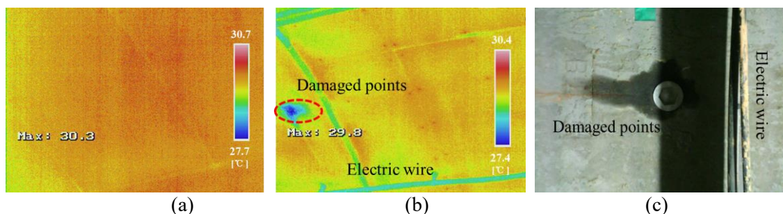
Figure 5. The filed detection results of thermal infrared camera: (a) the safety condition, (b) the leaking condition and (c) a leaking grouting hole in field.
