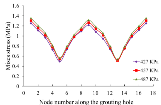
Figure 8. Mises stress along the grouting holes under different water pressure.
