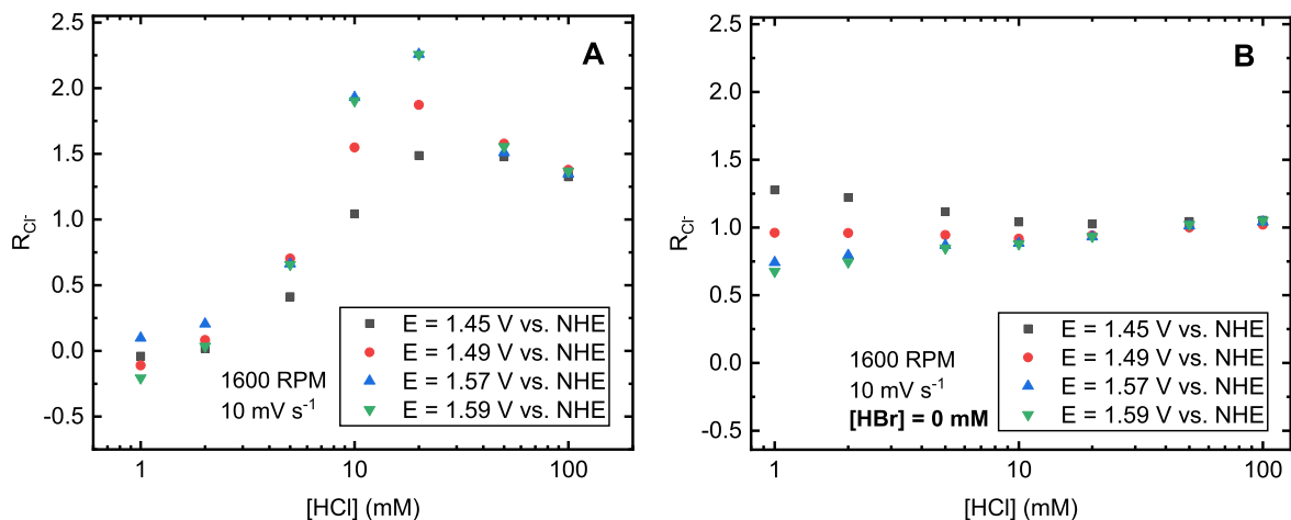
Figure 5. Chloride reaction order R_{\text{Cl}^-} as function of chloride concentration, based on data from Fig. 4b. Shown are values in presence of 10 mM HBr (a), as well as those in bromide-free conditions (b).
