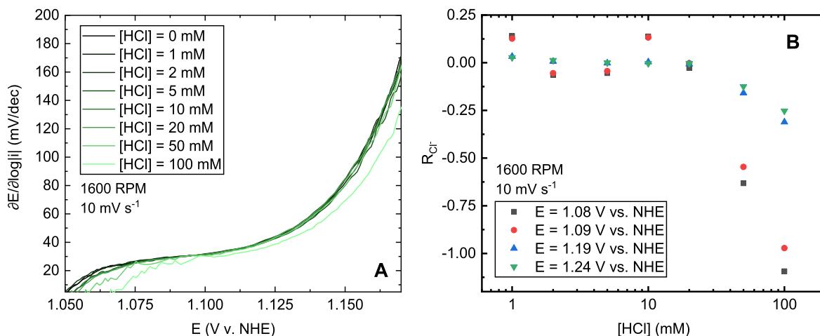
Figure 3. Tafel slope values in the bromide oxidation region of Fig. 2a for various measured chloride concentrations. Only forward scans are shown. B: Chloride reaction order R_{\text{Cl}^-} as function of chloride concentration, based on data shown in Fig. S 11B.
