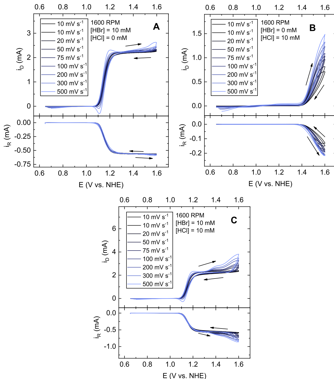
Figure 1. Cyclic voltammograms of a Pt-Pt RRDE in a solution of 0.1 M \text{HClO}_4 , showing the BER in presence of 10 mM HBr (Panel A), the CER in presence of 10 mM HCl (Panel B), and parallel oxidation of \text{Br}^- and \text{Cl}^- in presence of 10 mM HBr + 10 mM HCl (Panel C). Varying scan rates are shown in shades of blue at a fixed rotation rate of 1600 RPM. Top panels show disk currents, bottom panels show ring currents while keeping the ring potential at 0.7 V. Arrows indicate scan direction.
