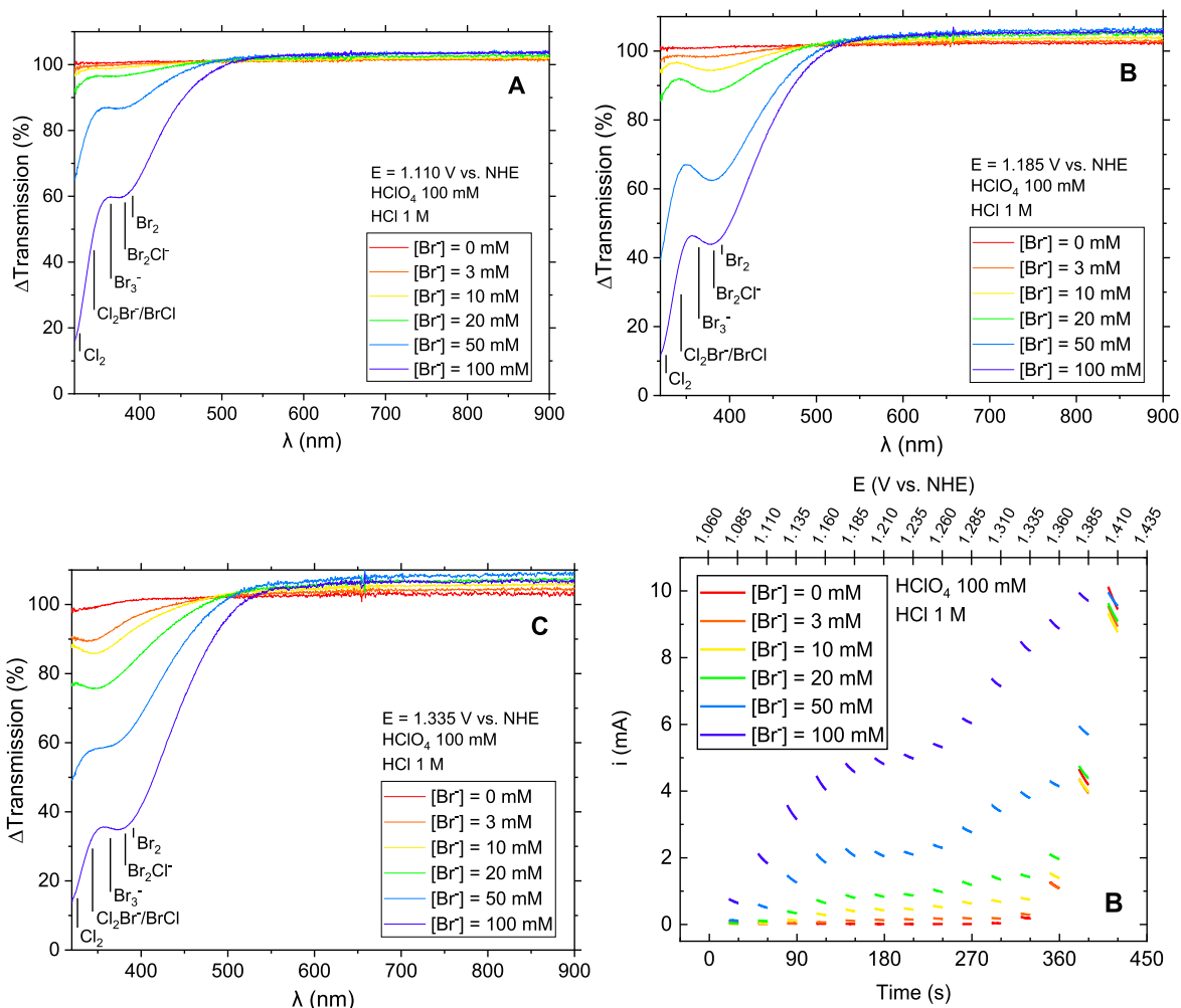
Figure 9. UV-vis measurements of a stationary Pt/FTO electrode in a solution of 0.1 M \text{HClO}_4 + 1 M \text{HCl} , in presence of various [\text{HBr}] . a, b and c: UV-vis spectra measured as function of bromide concentration, after stepping the potential up to 1.110 V (a), 1.185 V (b) and 1.335 V (c), in 25 mV steps of 30 s each. Spectra are shown of 10 s after applying the relevant potential. Previously published 47 wavelengths of peak adsorption are indicated for each relevant species. d: Corresponding currents measured during the experiments. Only the final 10 s of each potential step are shown for clarity (see Fig. S 30 for full data). Upper axis shows the potentials applied at each moment in time.
