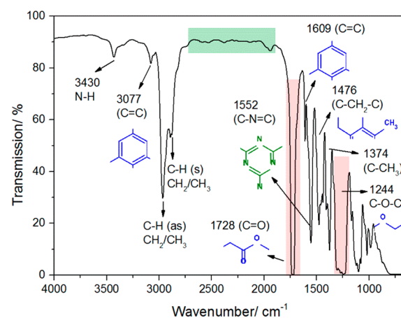
Figure 5. Transmission FTIR spectrum of 10 μm polyester coating.
