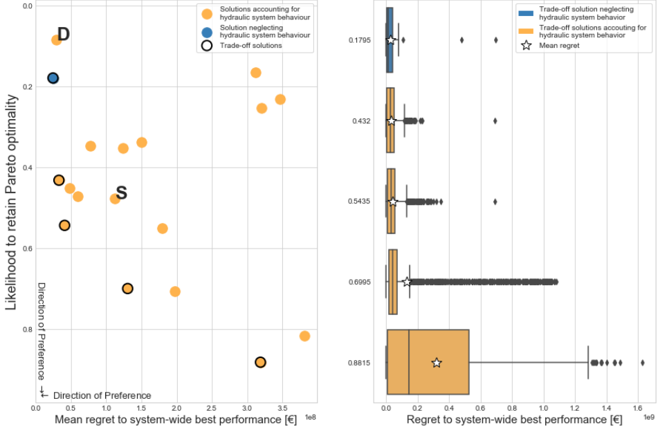
Figure 2.7 Left: Likelihood to retain Pareto optimality (y-axis) and mean regret relative to system-wide performances (x-axis) of all solutions. Right: boxplots of the regret relative to system-wide performances of the trade-off solutions.
