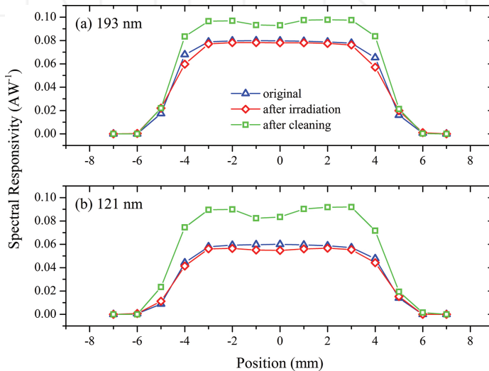
Figure 16. Measured responsivity across the surface in one direction of a 9.6 \times 9.6 \text{ mm}^2 LT PureB photodiode at wavelengths of 193 and 121 nm, before and after high-dose exposure, and after cleaning. The high-dose exposure was performed with a circular beam spot of \phi 1 \text{ mm} with a radiant exposure of 37 \text{ J/cm}^2 [22].
