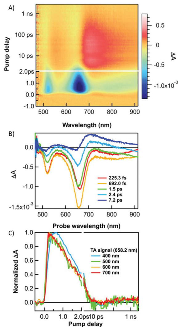
Fig. 4 (A) 2D transient absorption image showing the change in absorption (color coding) as a function of wavelength and time for InSb nanocrystals excited at 400 nm. (B) Spectral cuts at various times given in the legend showing the relative magnitudes of the bleach features at 660 nm and 520 nm. There is also photoinduced absorption developing at later times that obscures much of the bleach. (C) The time evolution of the bleach feature at probed at 660 nm at different excitation wavelengths, as indicated in the legend.
