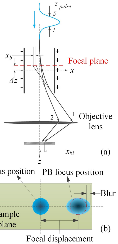
Fig. 3. Schematic indication of blur induced in an electron pulse by a beam blunker. (a) Electrons at the front of the electron pulse, indicated by 1, will undergo a different deflection and thus spot displacement than electrons at the rear of the pulse, indicated by 2. Note that the pulse is defined after the blanking aperture in the objective lens (dark gray) and the sketch indicates a slightly off-axis aperture. The different spot displacements in the pulse lead to a blur in the focus. x_b denotes the blur in the blunker and x_{bi} the blur on the sample plane: x_{bi} = M \cdot x_b . (b) Schematic depiction of the influence of blanking on the electron focus on the sample plane. CB: Continuous Beam; PB: Pulsed Beam. The amount of focal spot displacement depends on electrons in the center of the pulse, the blur is determined by the varying spot displacement within the pulse.
