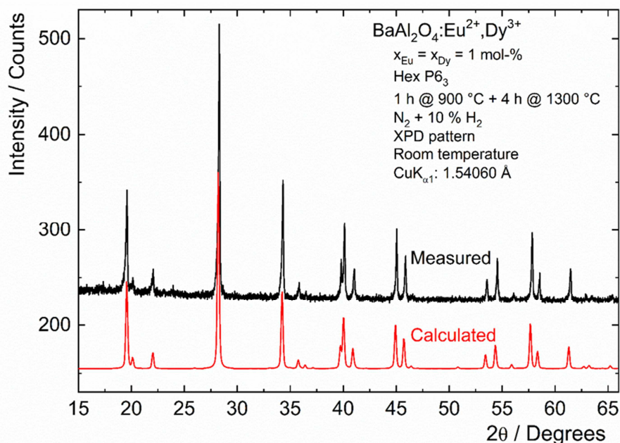
Figure 1. Measured and calculated [9,10] X-ray powder diffraction patterns of BaAl 2 O 4 :Eu 2+ ,Dy 3+ .
