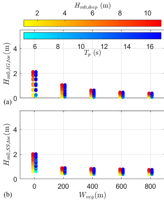
Fig. 19. Scatterplots of: (a) H_{m0,IG,toe} ; and (b) H_{m0,SS,toe} against W_{veg} ( \sigma=0^\circ , h_{toe}=1 m, \cot \alpha_{fore}=50 , n=0.012 s/m ^{1/3} , and \cot \alpha_{dike}=\infty ). Each data point is represented by two markers with colormaps indicating the magnitude of H_{m0,deep} (hot) and T_p (cold).
