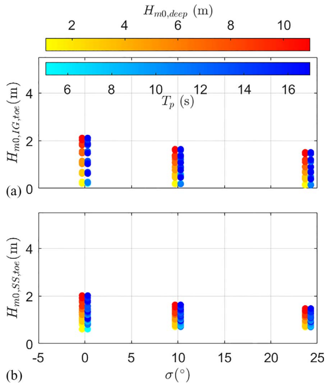
Fig. 11. Scatterplots of: (a) H_{m0,IG,toe} ; and (b) H_{m0,SS,toe} against \sigma ( h_{toe} = 1 m, \cot \alpha_{fore} = 50 , W_{veg} = 0 m, n = 0.012 s/m 1/3 , and \cot \alpha_{dike} = \infty ). Each data point is represented by two markers with color-maps indicating the magnitude of H_{m0,deep} (hot) and T_p (cold).
