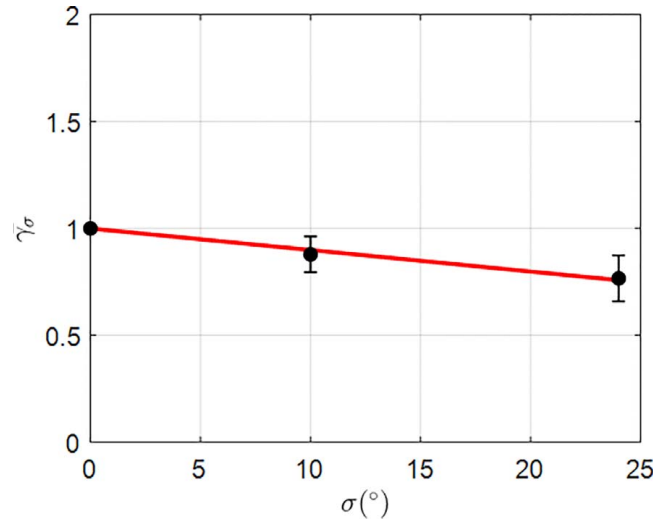
Fig. 12. Mean response of \hat{H}_{IG} to variations in \sigma , relative to the reference case ( \sigma = 0^\circ ). Line indicates the model fit [Eq. (26)]. Vertical error bars represent the standard deviation of each mean.
