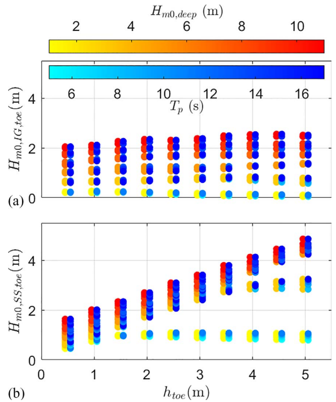
Fig. 13. Scatterplots of: (a) H_{m0,IG,toe} ; and (b) H_{m0,SS,toe} against h_{toe} ( \sigma = 0^\circ , \cot \alpha_{fore} = 50 , W_{veg} = 0 m, n = 0.012 s/m 1/3 , and \cot \alpha_{dike} = \infty ). Each data point is represented by two markers with color-maps indicating the magnitude of H_{m0,deep} (hot) and T_p (cold).
