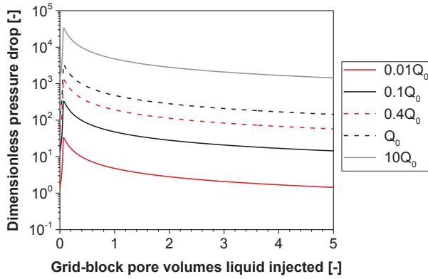
Fig. 11. Dimensionless pressure drop during liquid injection after 10 PV gas injection calculated from Peaceman equation. Liquid is injected at various injection rates ranging from 0.01Q_0 to 10Q_0 .
