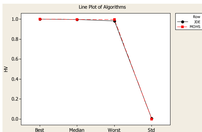
Figure 9. Line plot of HV volumes for both algorithms.
