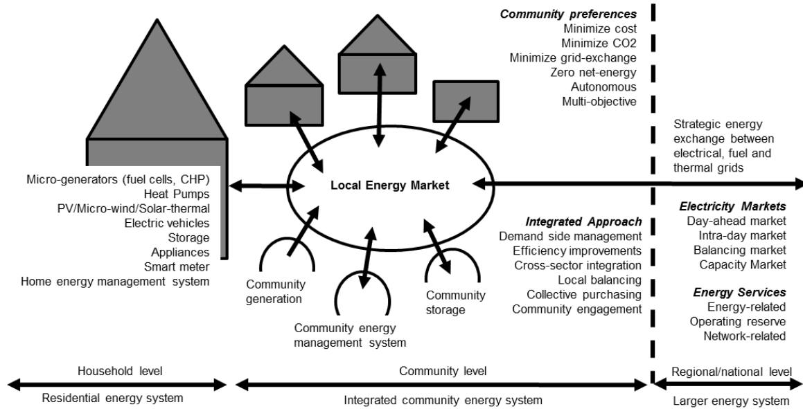
Figure 5. Functions of an integrated community energy system in the larger system
