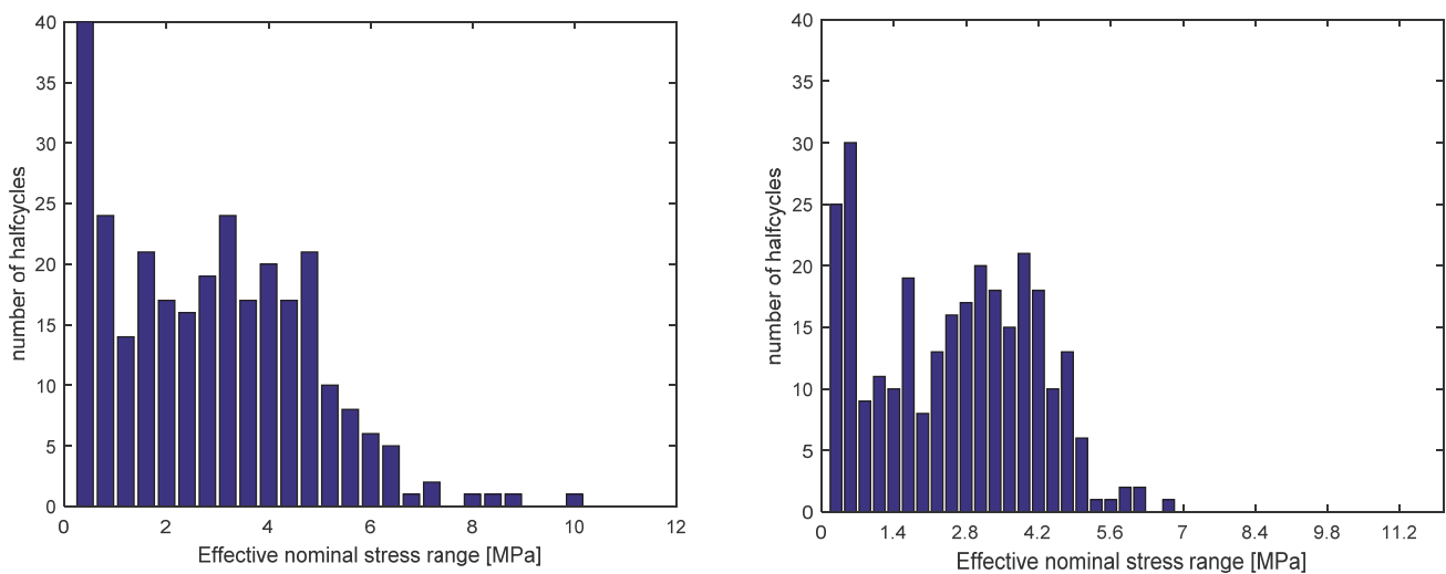
Figure 11: Histograms resulting from PDMR cycle counting of the load path depicted in Fig. 4 (right); Virtual path included (left) and excluded (right).
