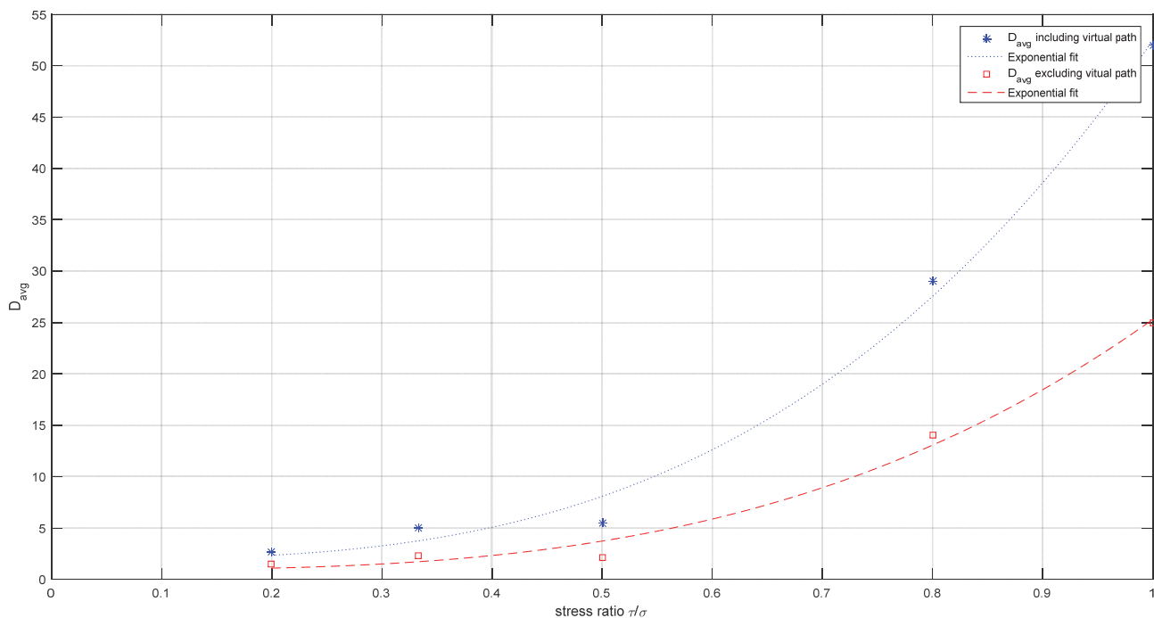
Figure 12: Graph showing the exponential increase of fatigue damage with increasing stress amplitude ratio considering PDMR based cycle counting
