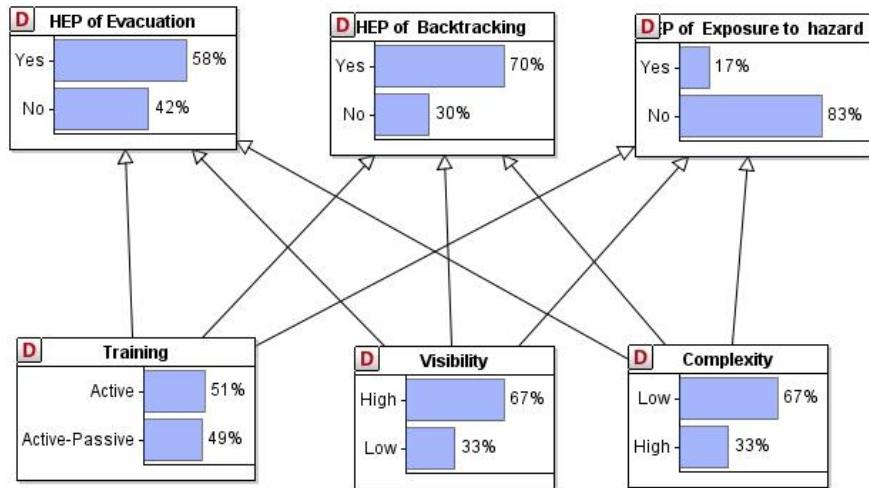
Figure 4. Developed BN via the learning parameter algorithm (BPL model).
