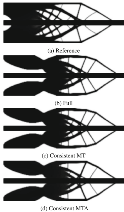
Fig. 3 Resulting cantilever designs of the mean eigenvalue maximization without peak constraint (a) and with peak constraint, solved by the full method (b) . The results of using reduced-order models with consistent sensitivities are shown for MT (c) and for MTA (d)
