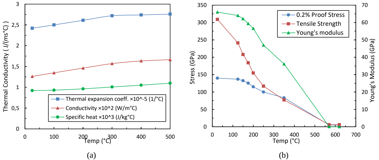
Fig. 19. (a) The physical and thermal properties of Al5083-H116 [30] (b) The mechanical properties of Al5083-H111 obtained from present investigation
