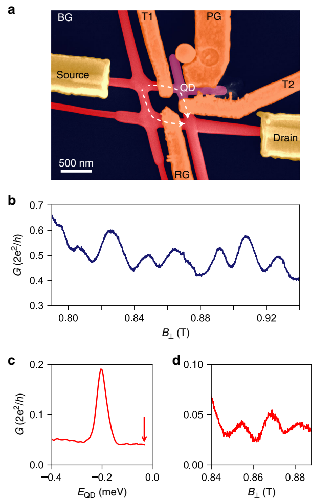
Fig. 2 Aharonov–Bohm oscillations in an InSb nanowire network. a False-colour scanning electron micrograph of the device: in red the nanowire network, in gold the leads, in orange the gates and in pink the quantum dot region. An additional illustration and a schematic of the device are shown in “Methods”. b Conductance at zero bias voltage G(V_{SD} = 0) as a function of the perpendicular field B_{\perp} in the open regime (i.e., with no QD defined) manifesting AB oscillations. c G(V_{SD} = 0) vs. E_{QD} (the dot electrochemical potential) when the quantum dot is defined. d G(V_{SD} = 0) vs. B_{\perp} when the dot is in the cotunnelling regime (cf. Coulomb valley indicated by the red arrow in (c)).
