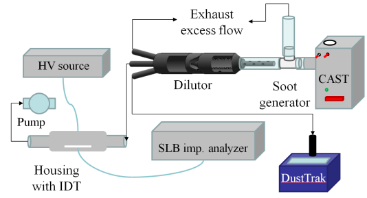
Fig. 3. A schematic overview of the measurement setup.
