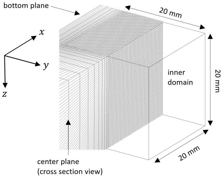
Figure 4.3: Cubic inner part ( 2\text{ cm} \times 2\text{ cm} \times 2\text{ cm} ) of the computational domain depicted in Fig. 4.1; the inner domain contains the bubble cluster depicted in Fig. 4.1.
