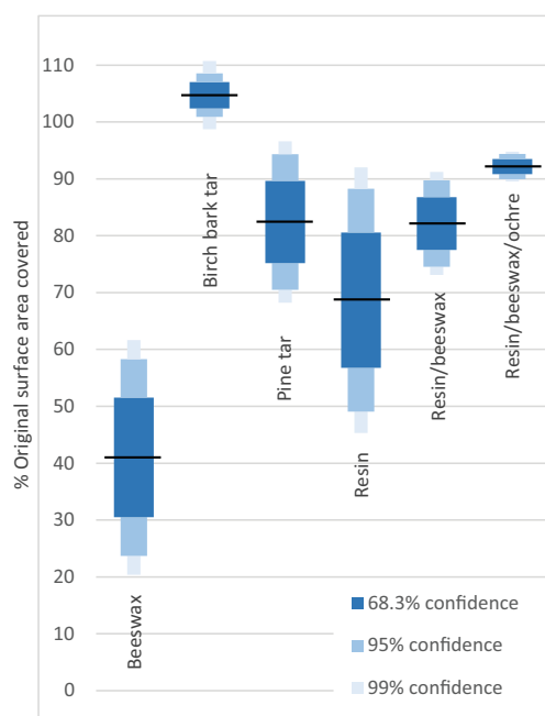
Fig. 7 Bullet graph displaying the error ranges for beeswax, birch tar, pine tar, resin, and resin/beeswax and resin/beeswax/ochre adhesives. Birch tar falls well outside the 99% confidence interval of the other adhesives
