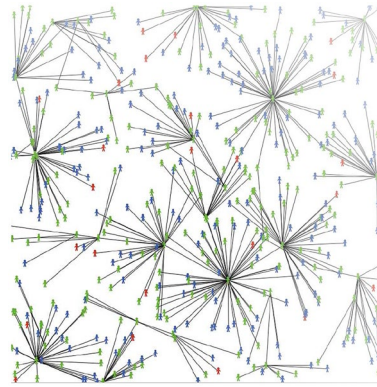
Fig. 1 An example of an emerged network of 500 nodes spread over an area of 25x25 with a transmission range of 5. The picture shows the visualization of the network in the simulation environment NetLogo (see Protocol evaluation and performance analysis)
