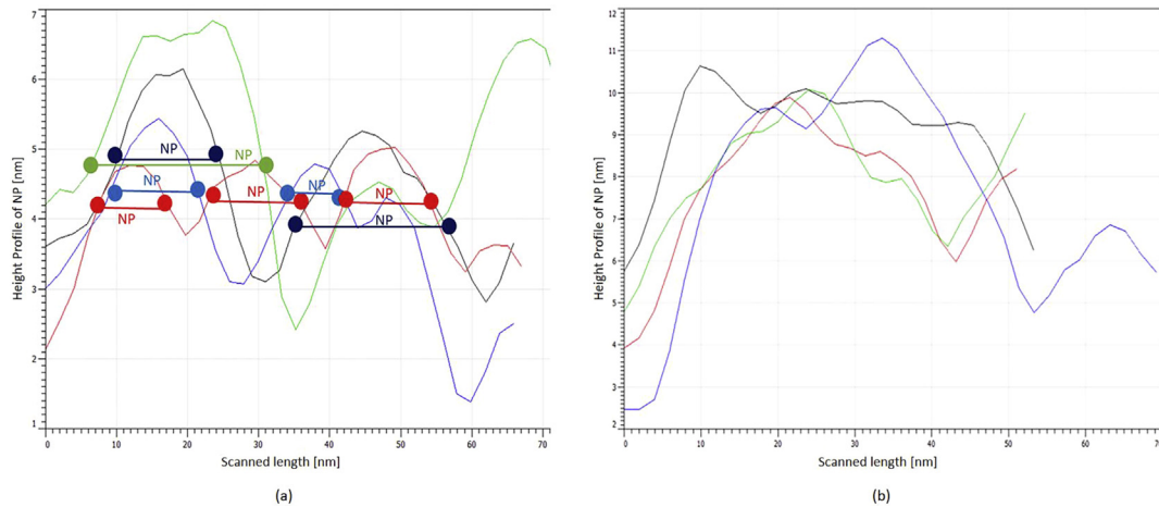
Fig. 3. Height profiles of the catalyst NP. (A) H_2 annealed NP (one height peak for each NP), (b) NH_3 annealed NP (several peaks for each cluster - not defined NP). (A colour version of this figure can be viewed online.)
