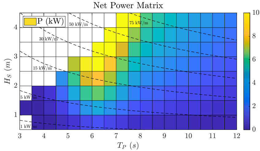
Fig. 15. Net Power Matrix for the MoonWEC device.
