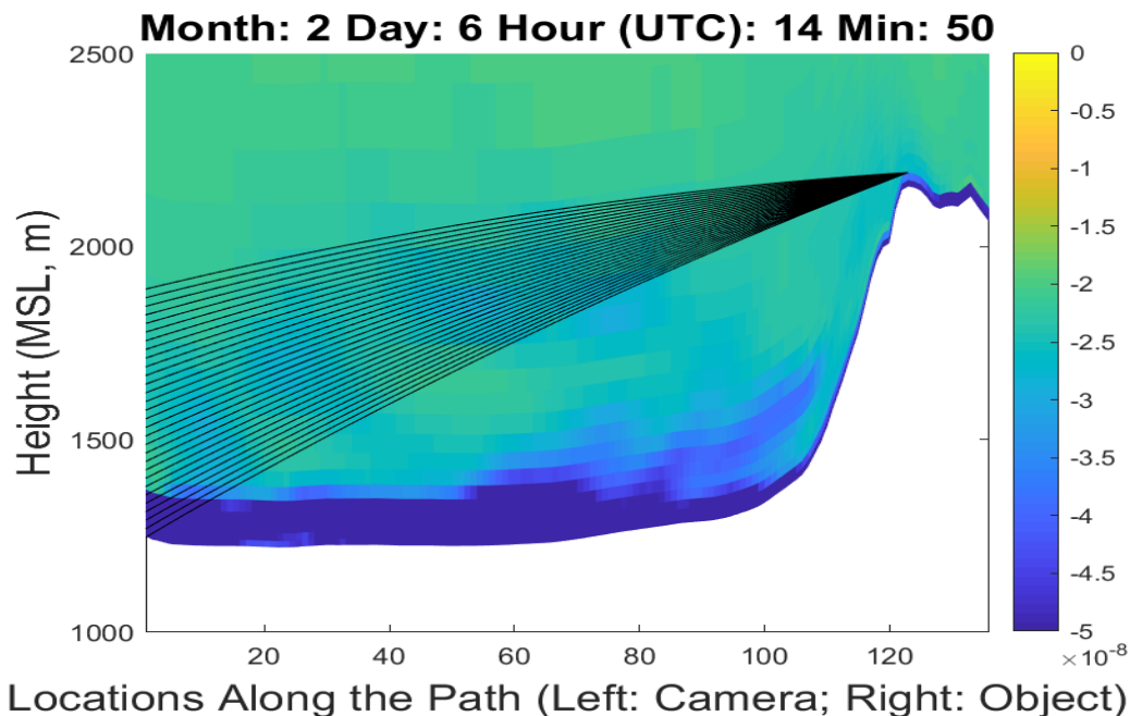
Figure 3. Example refractive index gradient results from numerical weather modeling for the WSMR experiment on February 6, 2018 at 14:50 UTC. The white area is the ground; the time-lapse camera is located in the basin on left side and a peak in the Oscura Mountains is on the right. Example ray tracing paths are shown between a position on the peak and the area near the camera.
