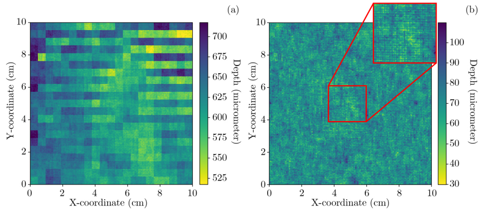
Fig. 3. Surface topology of a modern grounded canvas imaged with our multi-scale OCT approach. (a) Surface height before stitching. (b) Surface height after stitching. In an enlargement of the center part of the canvas, the regular pattern of the woven threads are clearly visible.
