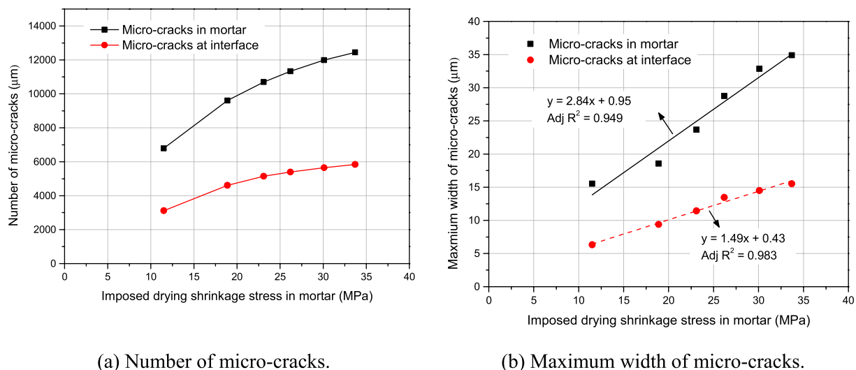
Fig. 12. Number and maximum width of micro-cracks in mortar and interface beams versus imposed drying shrinkage stresses in the mortar phase.
