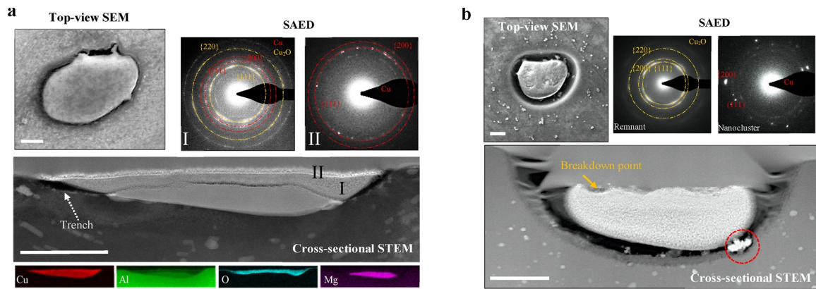
Fig. 5. Post-mortem analysis of corroded \text{Al}_2\text{CuMg} particles exposed to 0.01 M NaCl. (a) Top-view SEM, cross-sectional STEM/EDS and SAED analysis of an \text{Al}_2\text{CuMg} particle immersed in 0.01 M NaCl for 15 min. The SEAD patterns show characteristic rings and spots for Cu and \text{Cu}_2\text{O} ; the close lattice parameters are not indexed. (b) Top-view SEM, cross-sectional STEM and SAED analysis of an \text{Al}_2\text{CuMg} particle immersed in 0.01 M NaCl for 6 h. Note that the matrix and the particle are not at the same level where the nanoclusters nestled in the trench are identified as elemental copper. This undercut particle is a nano-porous \text{Cu}_2\text{O} remnant covered by \text{Al}(\text{OH})_3 . The cross-sections are fabricated out of the corresponding corroded particles with FIB. The scale bar is 1 \mu\text{m} .
