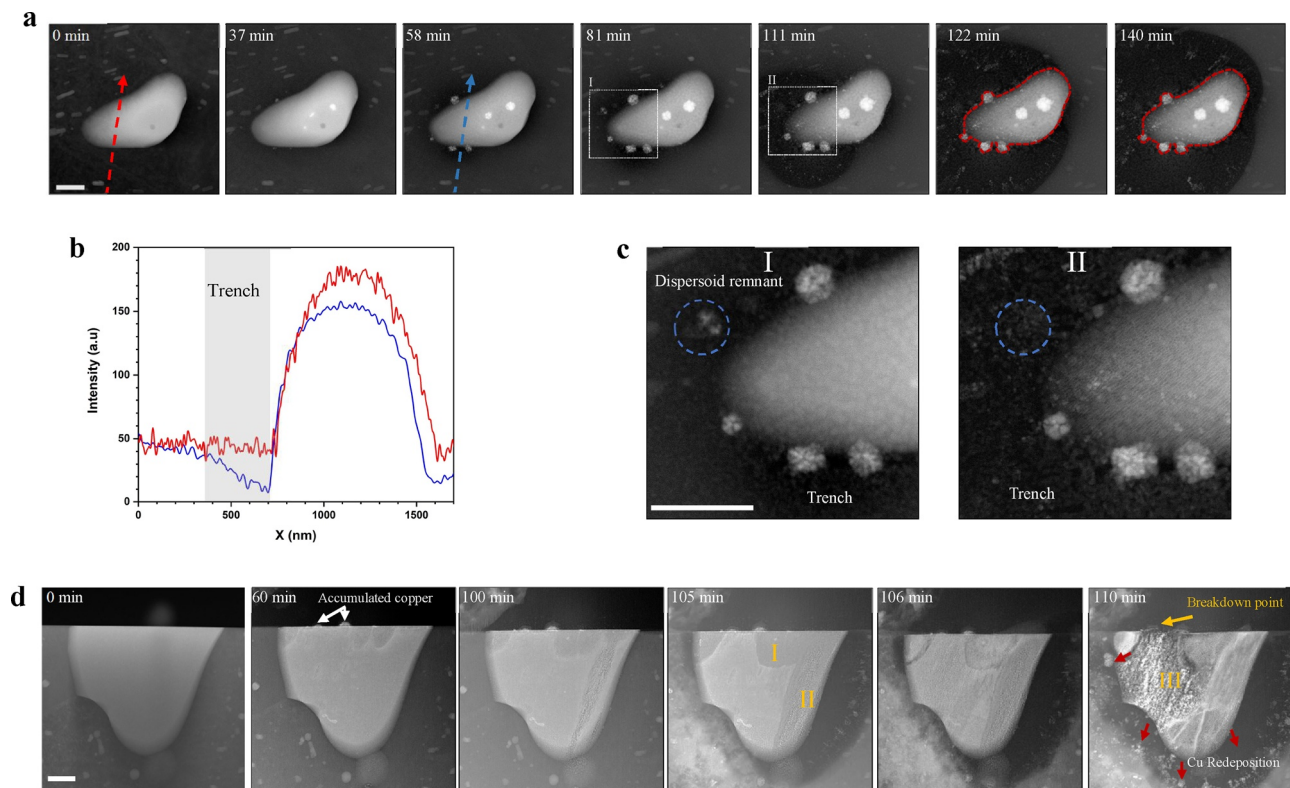
Fig. 6. In-situ top-view and cross-sectional-view observations of local corrosion by \theta -phase ( \text{Al}_2\text{Cu} ). (a) HAADF-STEM time series of top-view dealloying-driven evolutions within an \text{Al}_2\text{Cu} particle and its adjacent alloy matrix (Movie S4; it is made of 52 snapshots taken at different stages of an exposure for 149 min at the camera length of 75 mm). The red dashedlines indicate the particle area before and after the detachment. The lamella is approximately 200 nm thick, masked with 25-nm-thick TEOS layer on one side. (b) Electron intensity along the red and blue arrows in Fig. 6a, proving the trenching occurrence which follows the dealloying attack to the particle. (c) Digitally-magnified HAADF-STEM images of Region I and II in Fig. 6a, showing the transition from the globular to river-like dealloying morphology. The circled-in-blue region shows a dispersoid particle undergoing dealloying and then disappearing. (d) Cross-sectional dealloying-driven evolutions in a sandwiched \text{Al}_2\text{Cu} particle, captured by HAADF-STEM (Movie S5; Probe current in vacuum 1.409 nA, Convergence angle 13.7 mrad, Camera length 75 mm, Magnification 20000X). The total specimen thickness including TEOS layers is 350 nm. The white arrows point to the surface-diffused accumulation of copper. The yellow arrow points the breakdown location on the top of the particle. The red arrows indicate the copper dissolution merely from the periphery of the dealloyed particle at the trench bottom. The electrolyte is 0.01 M NaCl, pH 6.5. The scale bar is 500 nm. (For interpretation of the references to colour in this figure legend, the reader is referred to the web version of this article).
