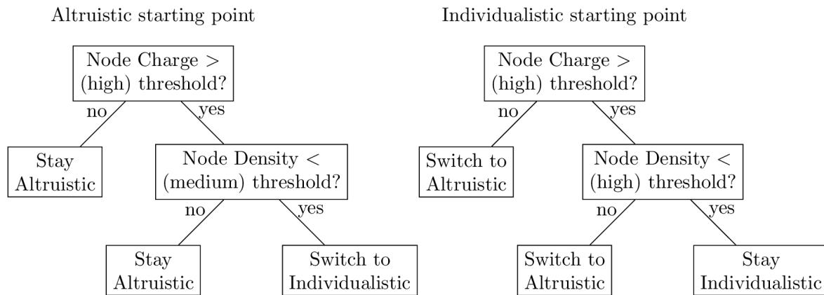
Figure 3: Decision tree for switching between altruistic to individualistic and back.
