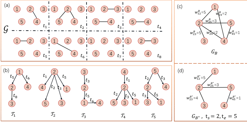
Figure 3.1: (a) A temporal network \mathcal{G} with N = 5 nodes and T = 8 time steps. (b) Spreading trees rooted at every seed node. The time step on each link denotes the time of the contact through which information diffuses. (c) The diffusion backbone G_B . (d) Diffusion backbone G_{B^*} confined within t_s = 2, t_e = 5 . When we consider the links that only appear in a time window [t_s, t_e] = [2, 5] , the value on the link shows the link weight in G_{B^*} .
