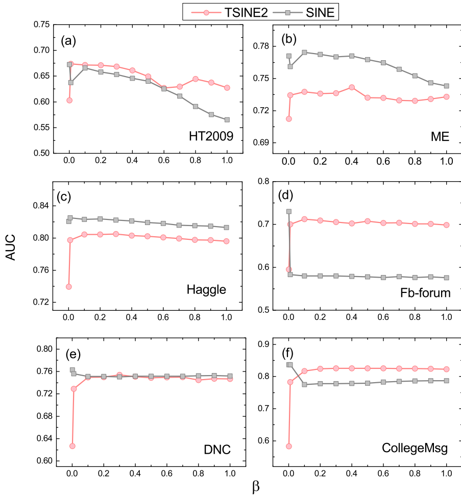
Figure 6.7: AUC as a function of \beta . We show the results for (a) HT2009 ; (b) ME ; (c) Haggle ; (d) Fb-forum ; (e) DNC ; (f) CollegeMsg .
