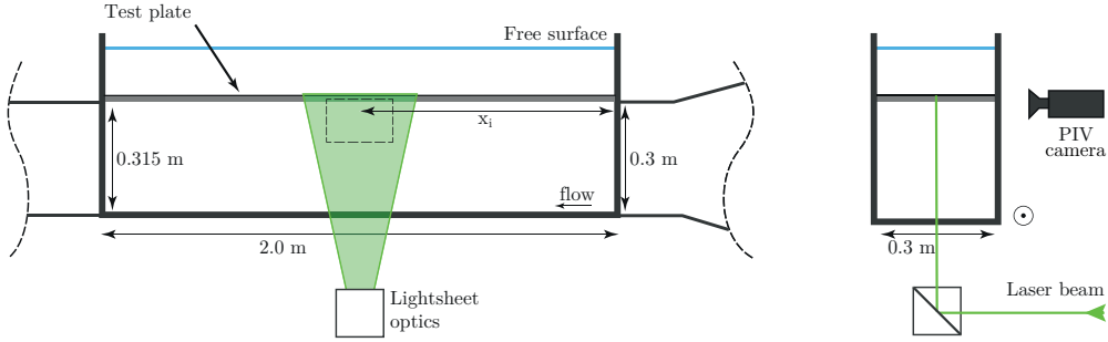
Figure 4.3: Illustration of the experimental PIV set-up applied to the test section of the facility. The field-of-views are located close to the wall at x_1 = 0.2 m, x_2 = 1.0 m and x_3 = 1.7 m from the leading edge of the test plate. The laser sheet is situated at the centerline of the water tunnel. The flow moves from right to left.
