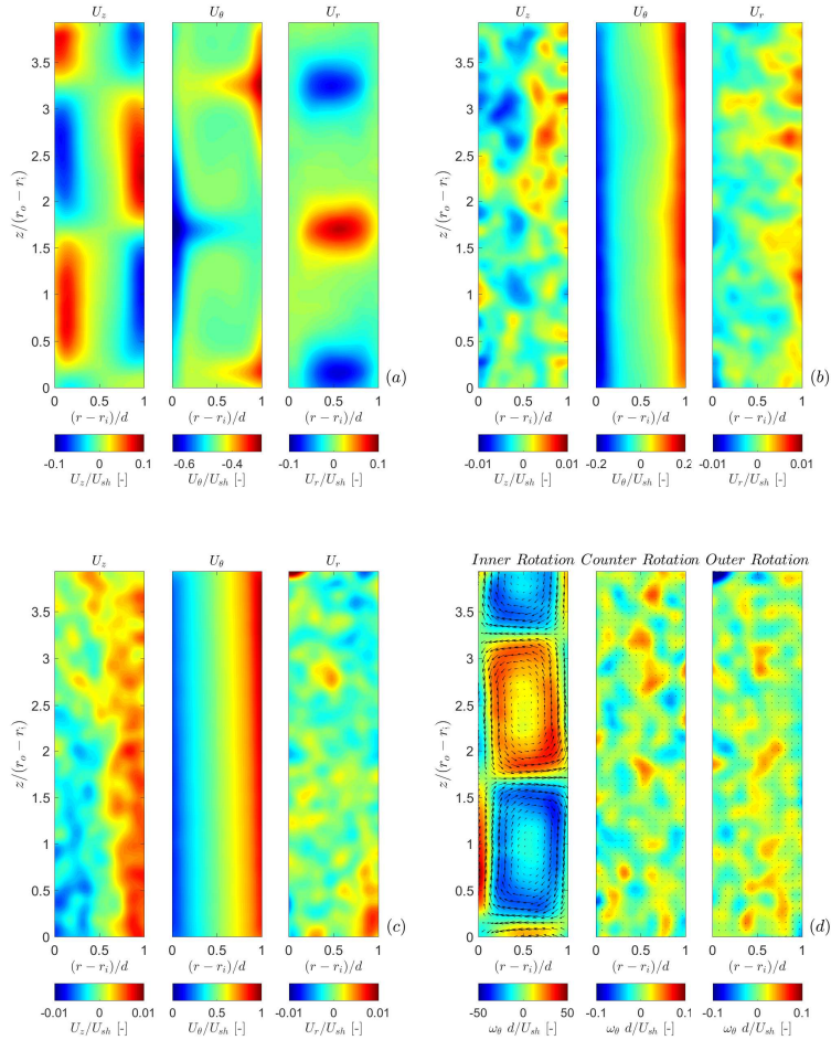
Figure A.2: Time-averaged normalised PIV results @ Reynolds number Re_s = 47000 for a) inner rotation R_\Omega = -0.083 , b) exact-counter rotation R_\Omega = 0 and c) outer rotation R_\Omega = 0.091 . The first panel indicates the axial velocity U_z , the second panel shows the azimuthal velocity U_\theta , while the third panel presents the radial velocity U_r . d) Out-of-plane vorticity for the three rotation conditions; color indicates the normalized strength, arrows indicate the radial and axial velocities.
