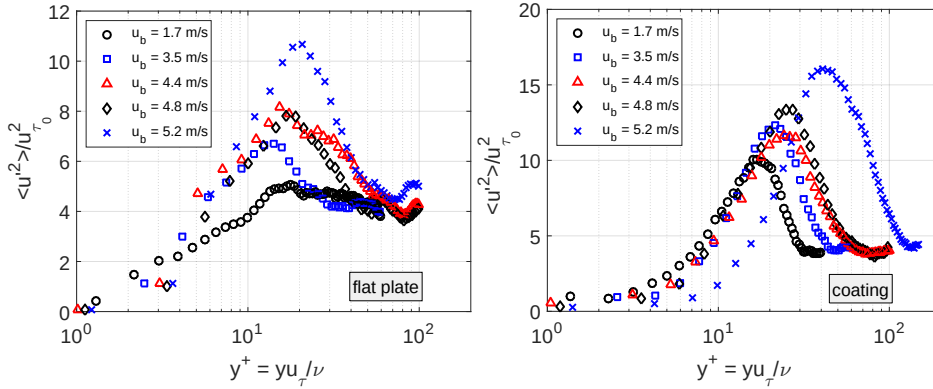
Figure 5.42: Dimensionless turbulent stress profiles \langle u'^2 \rangle reconstructed from the PTV results for bulk velocities U_b = 1.7 - 3.5 - 4.4 - 4.8 and 5.2 m/s. Left: flat smooth plate. Right: coated plate.
