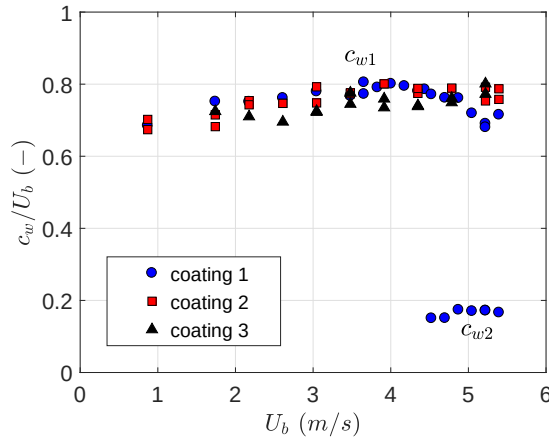
Figure 5.27: Surface wave velocity c_w/U_b as a function of the bulk velocity U_b .
