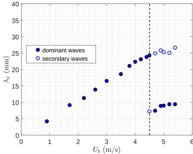
Figure 5.29: Wavelength \lambda_x of the dominant and the secondary waves in the one-way ( U_b < 4.5 m/s) and the two-way ( U_b > 4.5 m/s) coupled regime.
