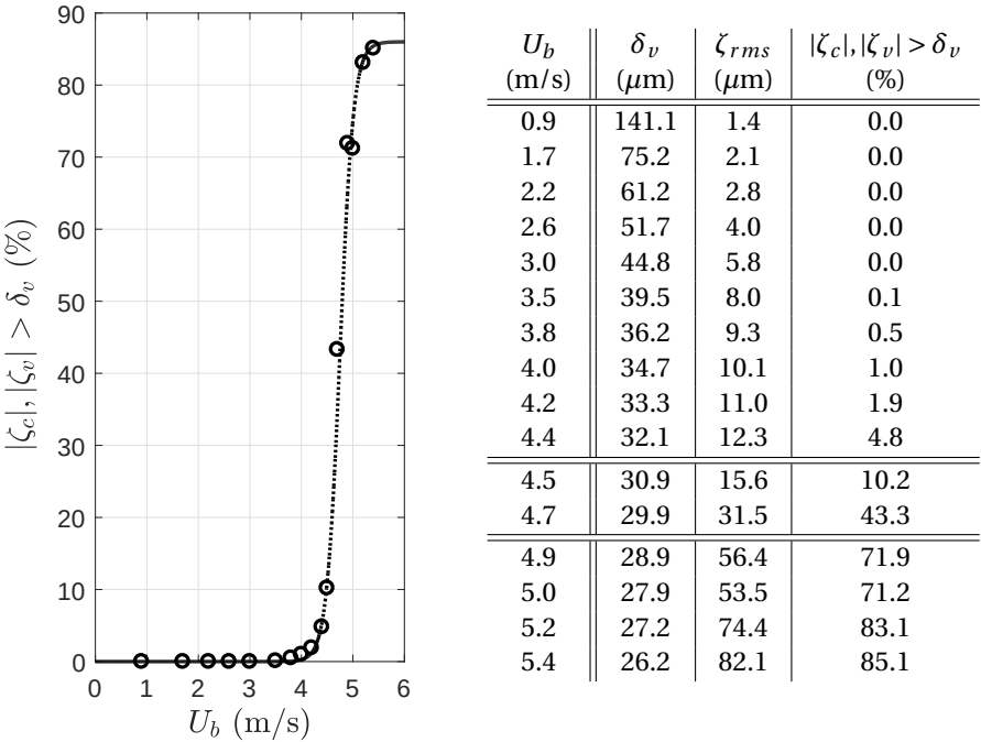
Figure 5.22: Figure (left) indicates the percentage of surface area that is covered with waves where the absolute value of the crest |\zeta_c| or the valley |\zeta_v| is respectively higher or lower than the viscous boundary layer \delta_v . The dotted line represents the data-fitted sigmoid curve. Table (right) presents the viscous boundary layer thickness \delta_v , the coating surface fluctuation \zeta_{rms} (coating 1) and the percentage of |\zeta_c|, |\zeta_v| > \delta_v related to the bulk fluid velocity U_b .
