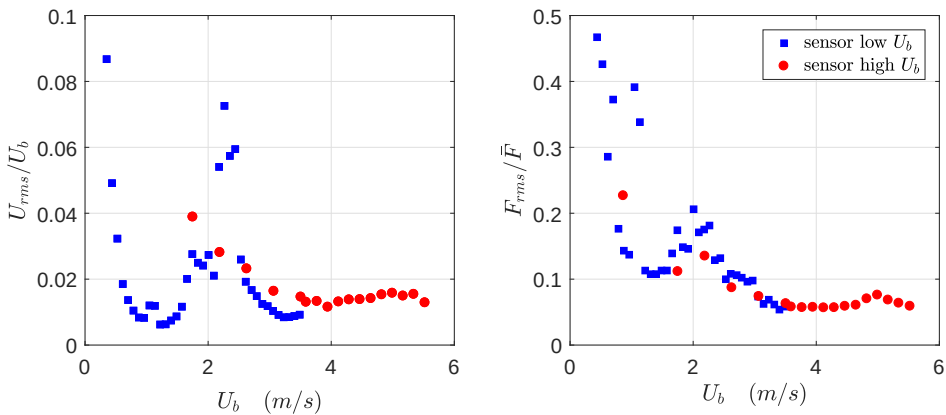
Figure 4.5: Root-mean-square (RMS) values based on the Gaussian fit of a) the velocity data and b) the force signals.
