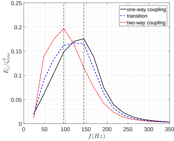
Figure 5.28: Surface displacement spectra E_\xi / \zeta_{rms}^2 as function of deformation frequency f . The three spectra correspond to the surface reconstruction results of bulk velocities U_b = 3.5 (black solid line), 4.5 (blue dashed line) and 5.4 m/s (red dash-dotted line), and represents the characteristic spectra for each regime.
