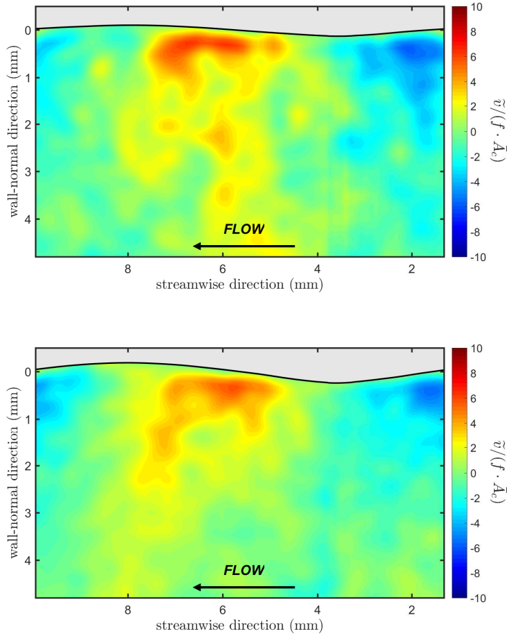
Figure 5.44: Wall-normal wave-induced velocity field \tilde{v} at bulk velocity U_b = 5.2 m/s of a) group 1, wave amplitude A_c = 0.1 - 0.2 mm and b) group 2, wave amplitude A_c = 0.2 - 0.4 mm.
