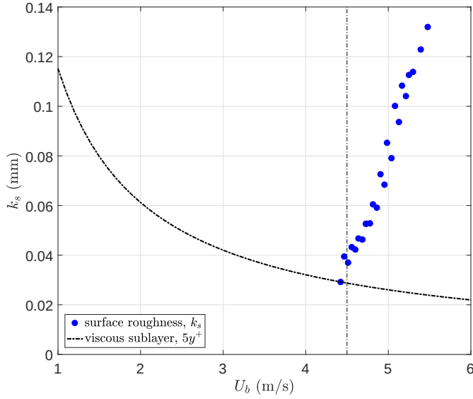
Figure 5.15: Estimated surface roughness k_s related to the measured drag coefficient C_d . The dot/dashed line represents the viscous sublayer thickness \delta_v = 5\nu/u_\tau , based on Grigson's correlation.
