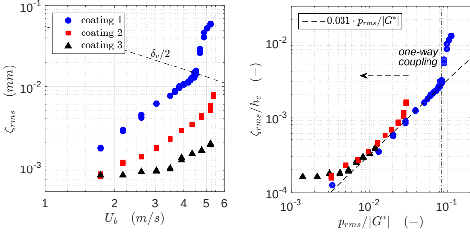
Figure 5.17: Vertical displacement of coating 1,2 & 3: a) Root-mean-square values \zeta_{rms} as a function of the bulk velocity U_b . The estimated 1-way/2-way regime transition of coating 1 occurs when the surface deformation is around \zeta_{rms} > \delta_v/2 . b) scaled RMS-values \zeta_{rms} to coating thickness h_c in relation to the scaled pressure fluctuations p_{rms} to coating shear modulus |G^*| . The scaling-factor 0.031 of the one-way coupled regime is a fit parameter which contains unknown factors, as discussed by Benshop et al. [10].
