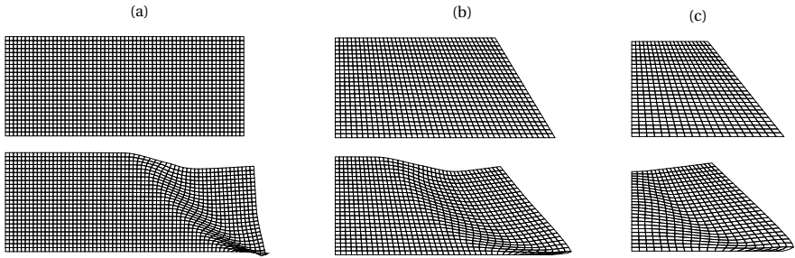
Figure 2.17: Initial and final mesh configurations after and before the a) 1 st Failure, b) 2 nd Failure, and c) 3 rd Failure
