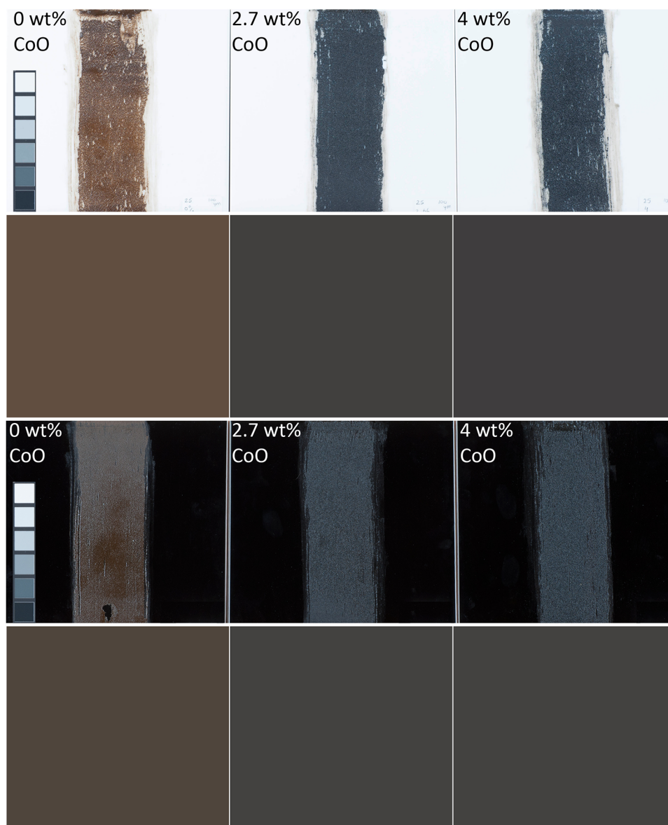
Fig. 6 Series of paint reconstructions of smalt mixtures based on sample x25 from Homer's belt (88 vol% smalt/glass, 5 vol% red earth, 5 vol% yellow earth, 2 vol% bone black), with colorless potash glass (0 wt% CoO), 2.66 wt% CoO smalt, and 4 wt% CoO smalt, applied on white and black tiles (1st and 3rd rows), with digital color reconstructions of the paint reconstructions based on the measured L*a*b* values to visualize the observed color differences (2nd and 4th rows)
