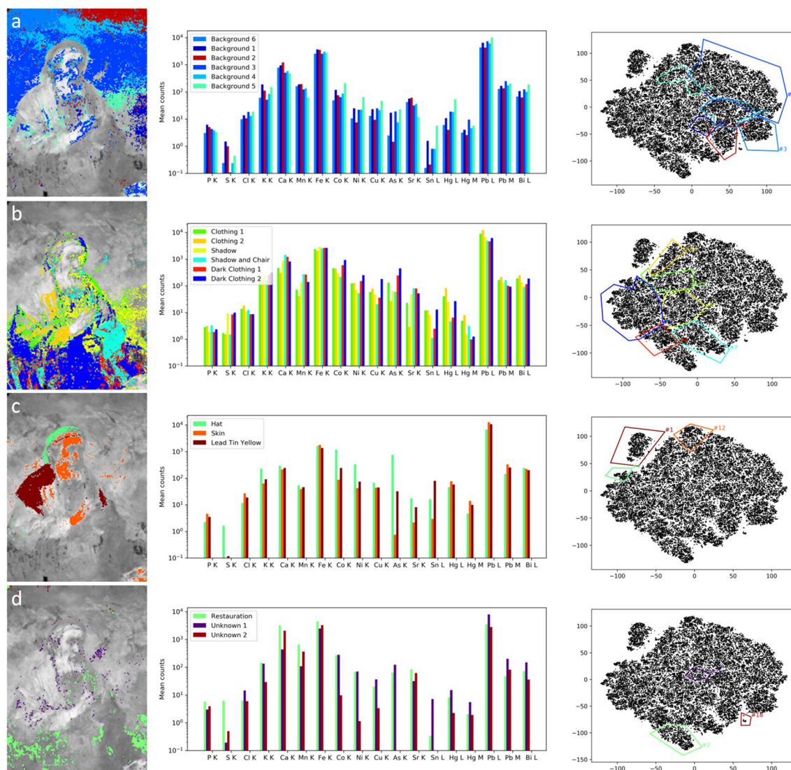
Fig. 3 T-SNE cluster analyses of the MA-XRF data showing the 18 clusters (a–d) as color projections on top of the Pb-L map (left), together with their spectral line intensities (middle), and tSNE plots (right)
