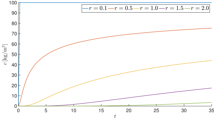
Figure 8.5: Plots of the concentrations of the bromide tracer c at z = 6.5 as function of the time t in seconds. Using the parameters: \alpha_r = 24.0 , \alpha_z = 1.0 and p_{\text{pump}} = 0.5 \cdot 10^5 .
