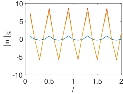
(d) The percentage change in the norm of the displacement, \gamma = 0.12 .
