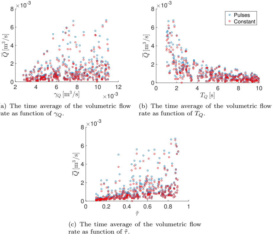
Figure 3.2: Scatter plots of the time average of the volumetric flow rate, after applying Monte Carlo simulations to the values of \gamma_Q , T_Q and \tilde{\tau} .
