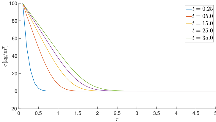
Figure 8.7: Plots of the concentrations of the bromide tracer c at z = 6.5 as function of the radius r in meters, for different times. Using the parameters: \alpha_r = 12.0 , \alpha_z = 1.0 and p_{pump} = 1.0 \cdot 10^5 .
