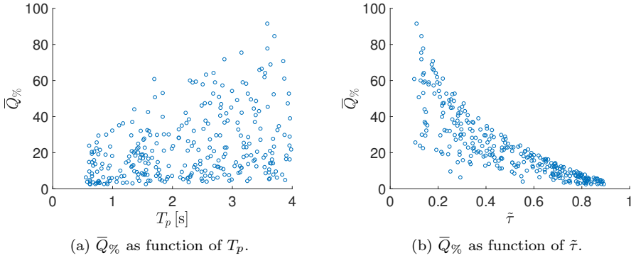
Figure 2.15: Scatter plots of the percentage change \bar{Q}_{\%} of the time average of the volumetric flow rate over the time interval (0, 20] , after applying Monte Carlo method to the values of T_p and \tilde{\tau} using the distributions (2.53). For the pump pressure, pulse waves (2.21) are used with p_{max} = 0.5 \cdot 10^5 Pa.
