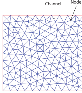
Figure 4.6: An illustration of a triangular unstructured network.
