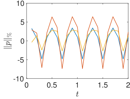
(b) The percentage change in the norm of the pressure, \gamma = 0.04 .
