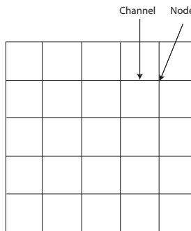
Figure 4.1: An illustration of a rectangular network.
