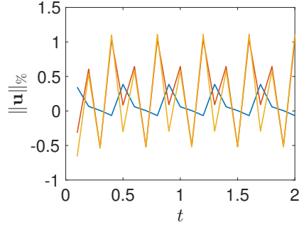
(b) The percentage change in the norm of the displacement, \gamma = 0.04 .
