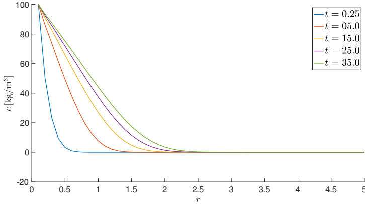
Figure 8.4: Plots of the concentrations of the bromide tracer c at z = 6.5 as function of the radius r in meters, for different times. Using the parameters: \alpha_r = 24.0 , \alpha_z = 1.0 and p_{\text{pump}} = 0.5 \cdot 10^5 .
