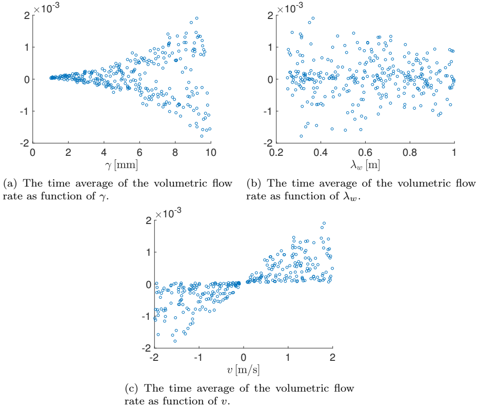
Figure 2.10: Scatter plots of the time average of the volumetric flow rate over the time interval (0, 70.86] , after applying Monte Carlo simulations to the values of \gamma , \lambda_w and v . For the vibrations transverse waves (2.16) are used as prescribed boundary displacement u_{vib} , with \gamma \sim \mathcal{U}(1, 10) mm, \lambda_w \sim \mathcal{U}(1/4, 1) m and v \sim \mathcal{U}(-2, 2) m/s.
