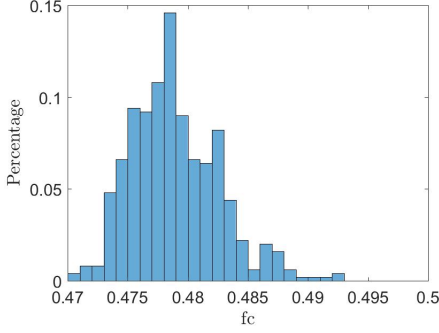
(a) The histogram of the fraction f_c that satisfies 0.05 < \kappa_n < 0.15 .
