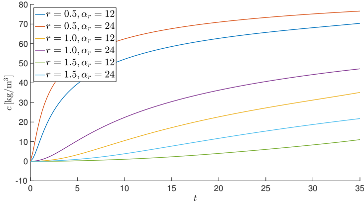
Figure 8.15: Plots of the concentrations of the bromide tracer c at z = 6.5 as function of the time t in seconds. Using the parameters: \alpha_z = 1.0 and p_{\text{pump}} = 0.5 \cdot 10^5 .
