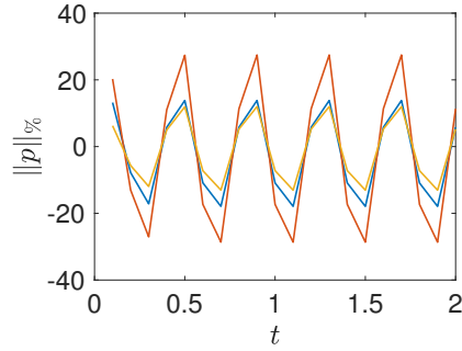
(d) The percentage change in the norm of the pressure, \gamma = 0.12 .
