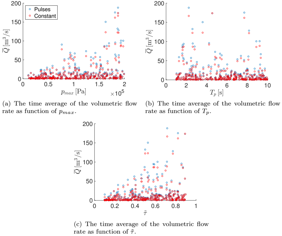
Figure 3.5: Scatter plots of the time average of the volumetric flow rate, after applying Monte Carlo simulations to the values of p_{max} , T_p and \tilde{\tau} .
