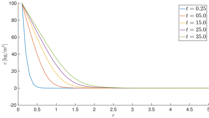
Figure 8.10: Plots of the concentrations of the bromide tracer c at z = 6.5 as function of the radius r in meters, for different times. Given a longitudinal dispersivity of 12.0 m, a transversal dispersivity of 1.0 m and a pump pressure of 0.5 \cdot 10^5 Pa.
