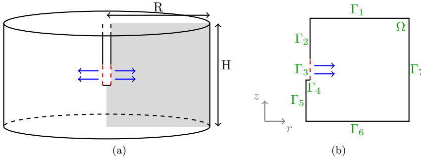
Figure 8.1: Sketch of the set-up for the aquifer problem: (left) physical problem and (right) numerical discretisation. Taking advantage of the symmetry of geometry and boundary conditions, only the grey region is discretised.
