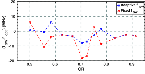
Fig. 8. Difference between the frequency at which the converter is operated and the optimum one in case of fixed and adaptive switching frequencies.
