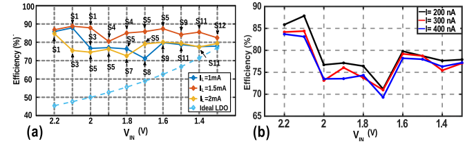
Fig. 17. Measured power efficiency versus V_{IN} for different values of (a) load current, and (b) biasing current of the gate driver circuit.
