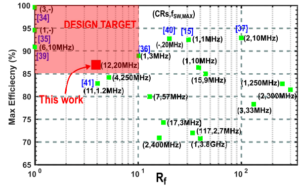
Fig. 20. Peak power efficiency of state-of-the-art DC-DC converters versus the ratio of maximum-to-minimum switching frequency ( R_f = \frac{f_{\text{SW,max}}}{f_{\text{SW,min}}} ). The number of implemented CRs, and f_{\text{SW,max}} are reported in the parenthesis.
