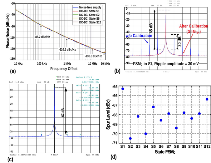
Fig. 21. (a) Measured oscillator PN performance at f = 5.5 \text{ GHz} and (b) its spectrum before and after calibration of the SRB with FSM C in State S1 and (c) State S5; (d) spur level across different converter states when the oscillator is calibrated only at State S1.
