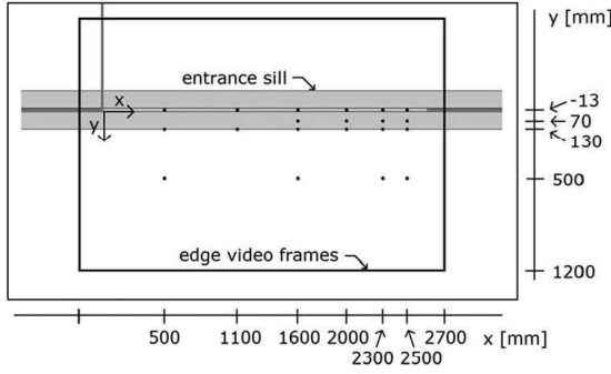
Figure 3. Locations of point measurements and the area of flow field measurements. The locations for point measurements are in front of and above the upward slope and crest of the sill with increasing density in downstream direction. The area of the flow field measurements depends on the video frames. The area of the video frames is in the middle of width the flume and covers the entire entrance sill area.
