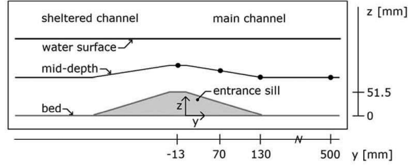
Cross section 2 - locations point measurements at mid-depth
