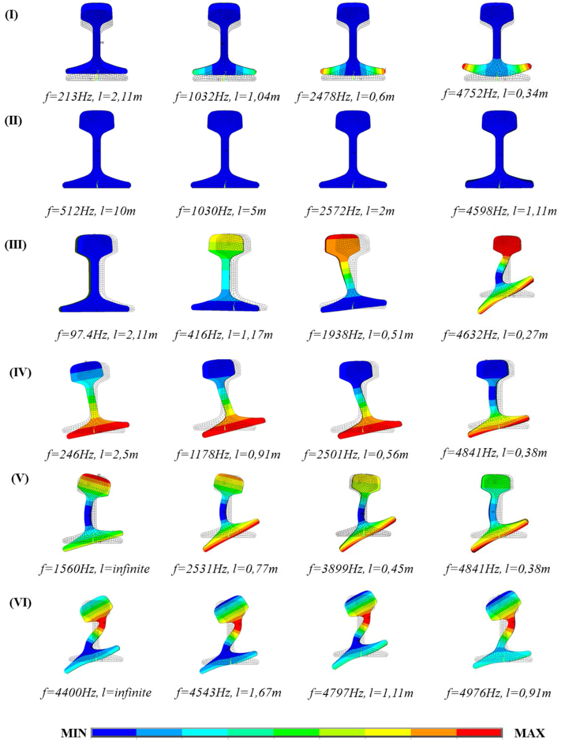
Fig. 3. Cross-sectional deformation of vertical bending modes (I), longitudinal compression modes (II), lateral bending modes (III), lateral torsion modes (IV), web 1 st bending modes (V), and web 2 nd bending modes (VI).
