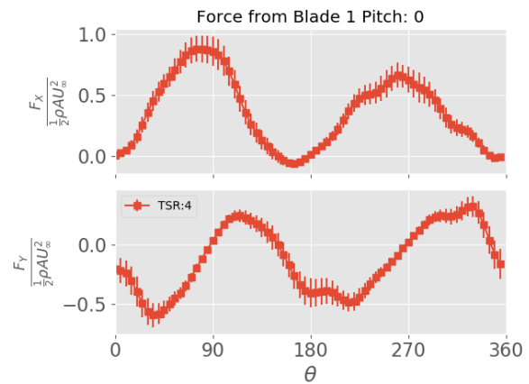
Figure 15. Blade 1 loading composed into X and Y directions
