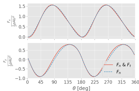
Figure 8. Thrust with and without F_t , \beta = 0^\circ
