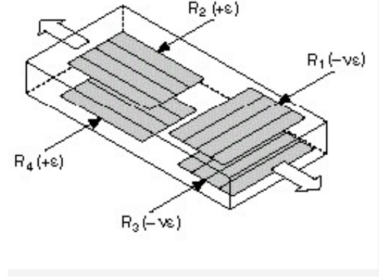
Figure 10. Strain gage configuration for measuring axial strain [7]
