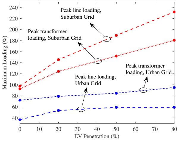
Fig. 6: Transformer and line loading trend as a function of EV penetration for Sub-urban and Urban grid.
