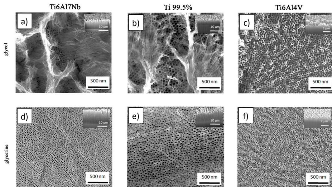
Figure 4. Top view and cross-section (insert) of anodic oxide layers on Ti6Al7Nb, Ti 99.5%, and Ti6Al4V alloys by anodization in glycol-based (a–c) and glycerol-based (d–f) electrolyte. In the top view, the scale bar corresponds to 500 nm for every substrate. In the cross-section, the scale bar represents 10 \mu\text{m} for Ti6Al7Nb and Ti 99.5%, and 2 \mu\text{m} for Ti6Al4V.
