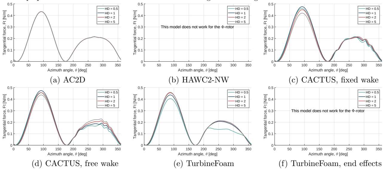
Figure 7: Tangential blade force vs the azimuth angle using six different models for the three-bladed \Phi -turbine with an aspect ratio of 0.5, 1, 2 or 5. The rotor solidity is 0.085 and the tip speed ratio is 3. The loads are shown for the mid-plane.
