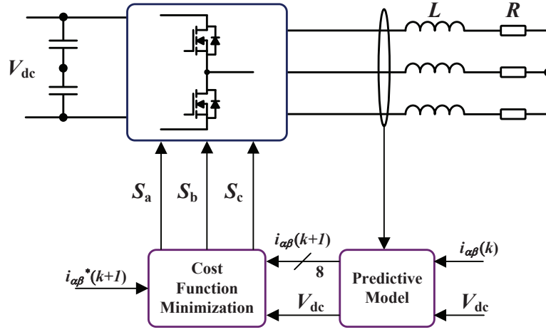
Fig. 2: Block diagram of a conventional FCS-MPC.
