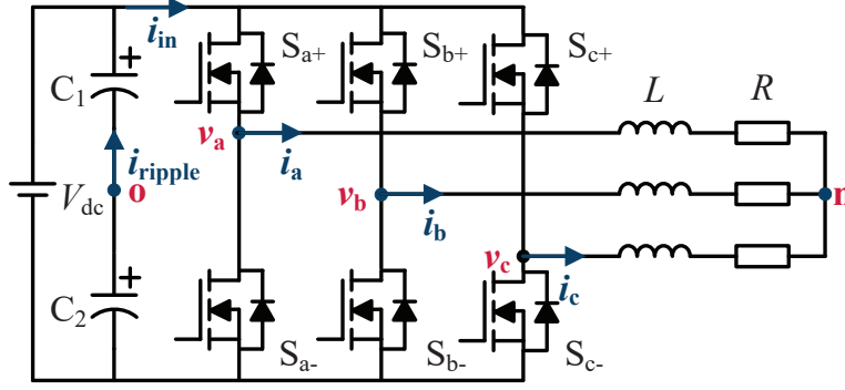
Fig. 1: Circuit schematic of the three-phase three-wire two-level VSI.
