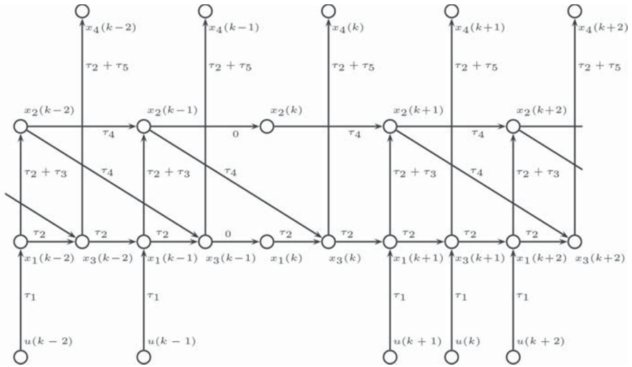
Fig. 5 Dynamic graph of the printer paper flow system of Section 3.2 in duplex mode in the cycles k - 2, k - 1, k + 1, \text{ and } k + 2 , but in simplex mode in cycle k
