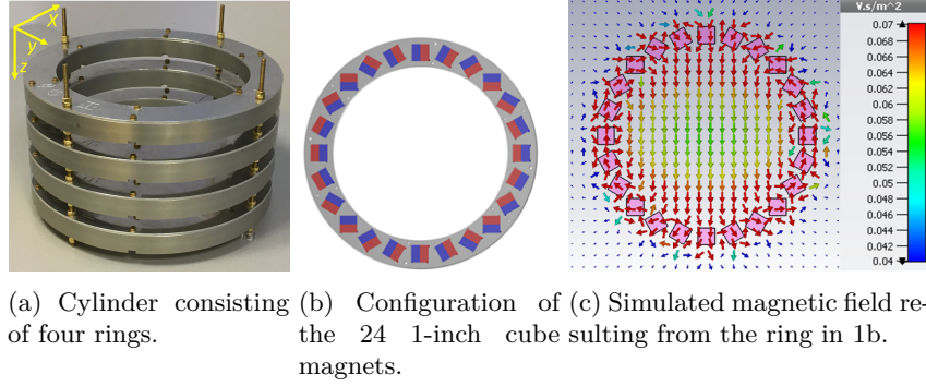
Fig. 1: Halbach cylinder, magnets and magnetic field.
