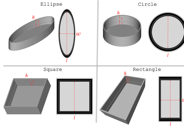
Fig. 6: The height h , length l , and width w illustrated for each shape. For each geometric shape, variations are made with the same height but with different length and width, see Table 1. This is done to make the dataset as diverse as possible.
