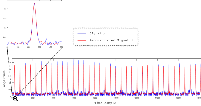
Fig. 9: The measured time signals (blue) plotted against the reconstructed signals (red) for each angle. The measured signal corresponds to the first measured sample, Sample_1.
