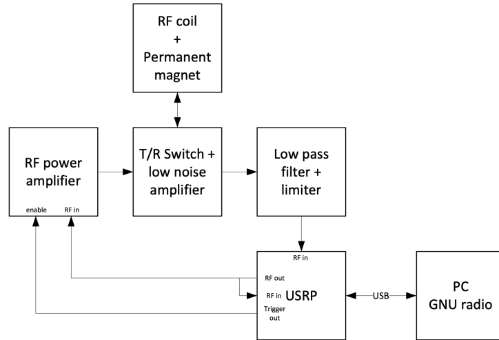
Fig. 4: Block diagram representing the MRI system
