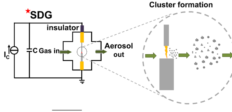
Figure 1. Schematic of the system for cluster formation by SDG showing the electrical circuit and the spark housing (cross-shaped block), I_c is the constant current to charge the capacitor C ; The magnified region between the two electrodes is showing a cartoon of the particle formation process.
