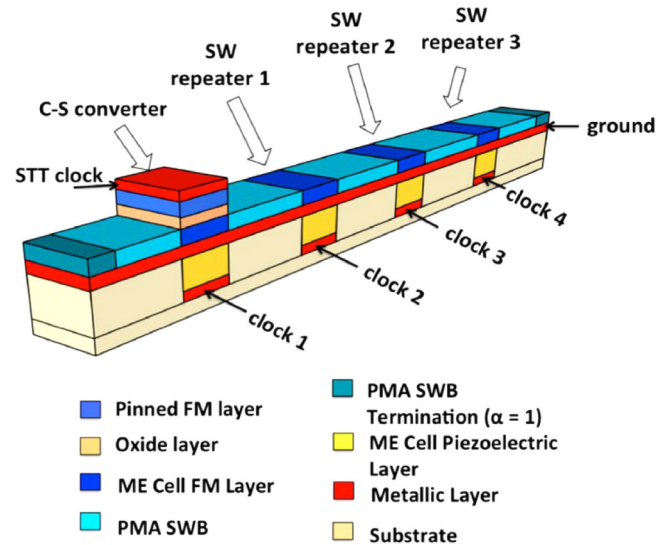
FIG. 8. Schematic of a clocked spin-wave interconnect. Reproduced with permission from S. Dutta, S.-C. Chang, N. Kani, D. E. Nikonov, S. Manipatruni, I. A. Young, and A. Naeemi, Sci. Rep. 5 , 9861 (2015). Copyright 2015 Nature.
