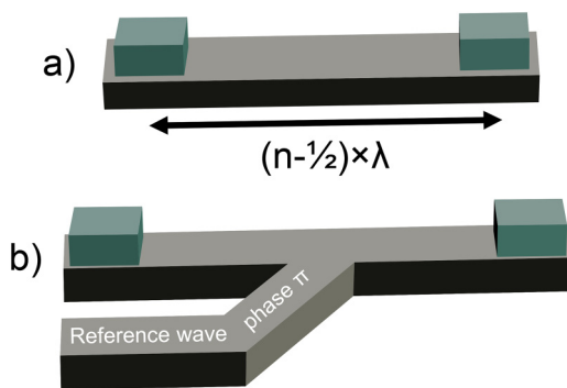
FIG. 16. Implementation of spin-wave inverters. (a) Phase encoding: inversion occurs by propagation along a “delay line” with a length of (n - \frac{1}{2}) \times \lambda , with \lambda being the spin-wave wavelength and n = 1, 2, 3, \dots an integer. (b) Amplitude encoding: inversion occurs by interference with a reference wave with phase \pi .
