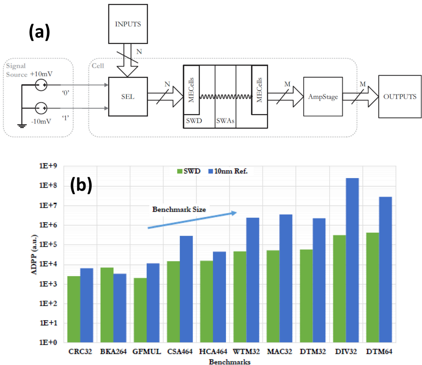
FIG. 24. Benchmark of hybrid spin-wave-CMOS systems. (a) Schematic of the hybrid system. Reproduced with permission from Zografos, P. Raghavan, L. Amari, B. Sorée, R. Lauwereins, I. Radu, D. Verkest, and A. Thean, in 2014 IEEE/ACM International Symposium on Nanoscale Architectures (NANOARCH) (2014) pp. 25–30. Copyright 2014 IEEE. (b) Area-delay-power (ADP) product of several arithmetic circuits (see the text) implemented in hybrid spin-wave-CMOS technology as well as 10 nm CMOS as a reference. Reproduced with permission from O. Zografos, B. Sorée, A. Vaysset, S. Cosemans, L. Amari, P.-E. Gaillardon, G. D. Micheli, R. Lauwereins, S. Sayan, P. Raghavan, I. P. Radu, and A. Thean, in 2015 IEEE 15th International Conference on Nanotechnology (IEEE-NANO) (2015) pp. 686–689. Copyright 2015 IEEE.
