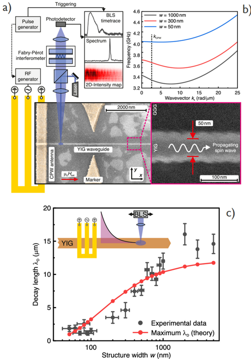
FIG. 13. (a) Schematic of the BLS experimental configuration and scanning electron micrographs of a 50 nm wide YIG conduit. (b) Spin-wave dispersion relations for YIG waveguides with different widths ( w = 1000, 300, 50 nm) in the backward volume geometry. (c) Experimental spin-wave attenuation (decay) length vs structure width. Reproduced with permission from B. Heinz, T. Brächer, M. Schneider, Q. Wang, B. Lägler, A. M. Friedel, D. Breitbach, S. Steinert, T. Meyer, M. Kewenig, C. Dubs, P. Pirro, and A. V. Chumak, Nano Lett. 20 , 4220 (2020). Copyright 2020 American Chemical Society.
