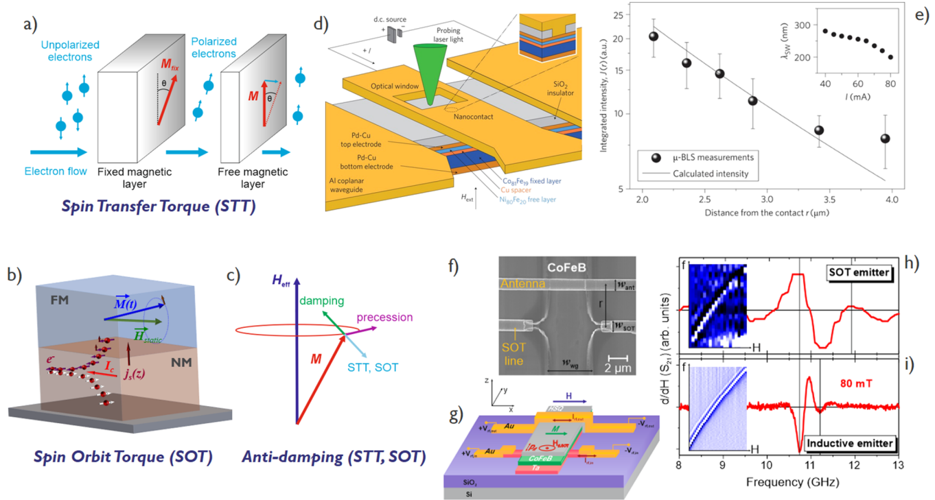
FIG. 10. Schematic illustrations of (a) spin-transfer torque (STT) and (b) spin-orbit torque (SOT) processes. (c) Magnetization dynamics in an effective field including precession, damping, and both STT and SOT. (d) Device layout used for the excitation of spin waves by STT. Reproduced with permission from M. Madami, S. Bonetti, G. Consolo, S. Tacchi, G. Carlotti, G. Gubbiotti, F. B. Mancoff, M. A. Yar, and J. Åkerman, Nat. Nanotechnol. 6 , 635 (2011). Copyright 2020 Springer Nature. (e) Attenuation of the excited spin waves during propagation. Reproduced with permission from M. Madami, S. Bonetti, G. Consolo, S. Tacchi, G. Carlotti, G. Gubbiotti, F. B. Mancoff, M. A. Yar, and J. Åkerman, Nat. Nanotechnol. 6 , 635 (2011). Copyright 2020 Springer Nature. (f) Scanning electron micrograph and (g) schematic layout of a device based on an SOT emitter and an inductive antenna detector. (h) and (i) Intensity of spin waves generated by a SOT antenna [(h), magnified 20 \times ] and an inductive antenna (i). Reproduced with permission from G. Talmelli, F. Ciubotaru, K. Garello, X. Sun, M. Heyns, I. P. Radu, C. Adelman, and T. Devolder, Phys. Rev. Appl. 10 , 044060 (2018). Copyright 2018 American Physical Society. The plots show the magnetic-field derivative of the forward-transmission S-parameter, dS_{21}/dH (emitter-to-detector distance 4 \mu\text{m} , applied magnetic field \mu_0 H = 80 mT). The insets show field–frequency signal maps corresponding to spin waves emitted by the two types of antennas (magnetic fields \mu_0 H = 52 –145 mT, frequencies 8–15 GHz).
